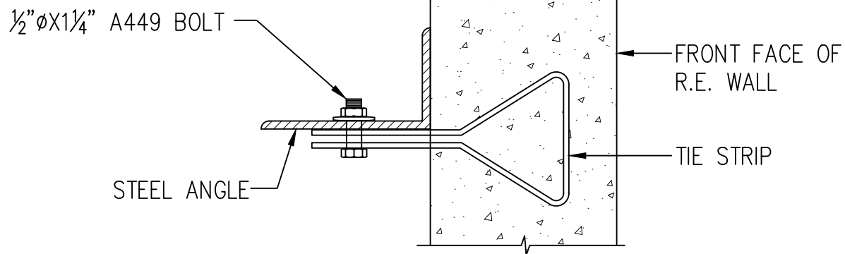
DETAIL ① ANGLE BOLTED TO TIE STRIP
