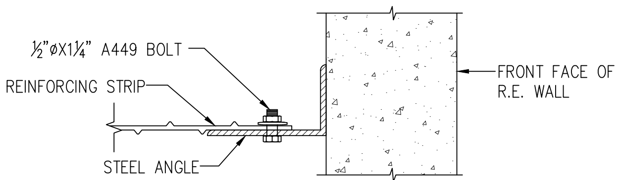
DETAIL ② SHIFTED REINFORCING STRIP BOLTED TO ANGLE
