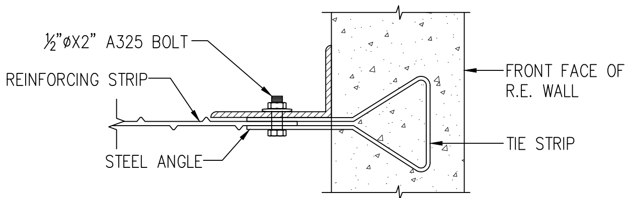
DETAIL ③ REINFORCING STRIP AND ANGLE BOLTED TO TIE STRIP
