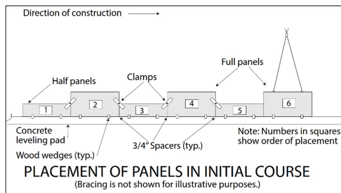
Figure 19: Placement of initial panel course.
