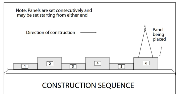
Figure 14: Use of spacer block to set panel spacing.
