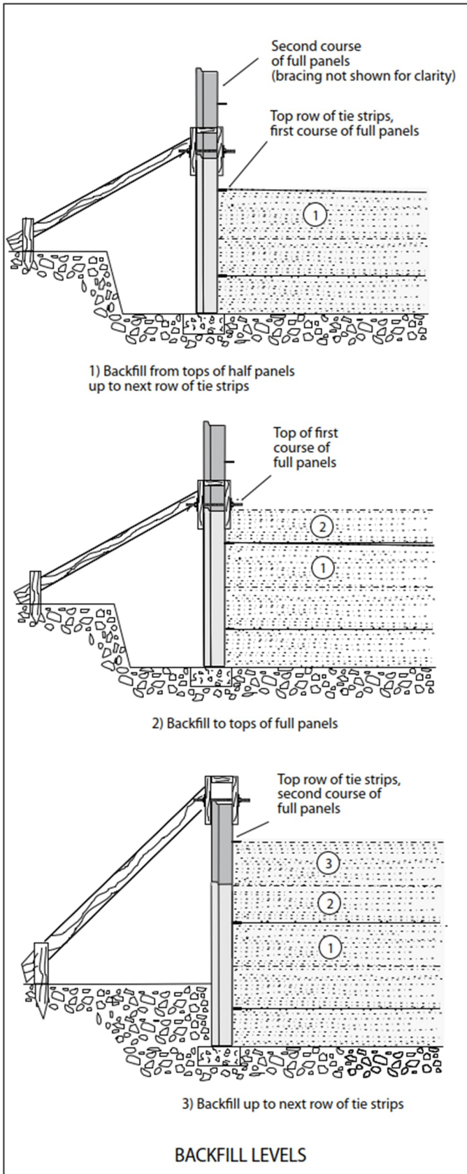
Figure 30: Backfill levels.
