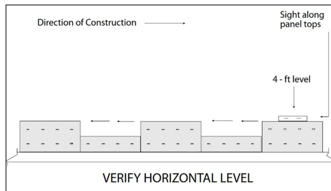
Figure 16: Verify horizontal level
