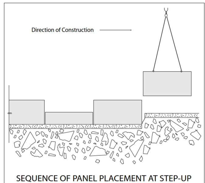
Figure 28: Sequence of panel placement at leveling pad step.
