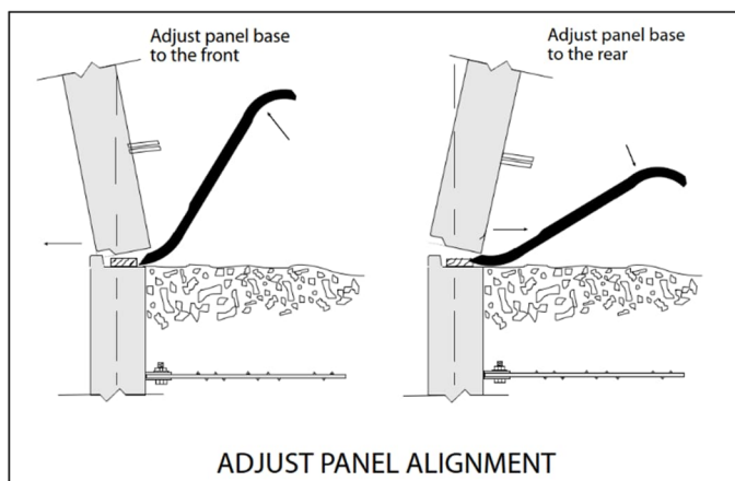
Figure 15: Adjusting panel alignment
