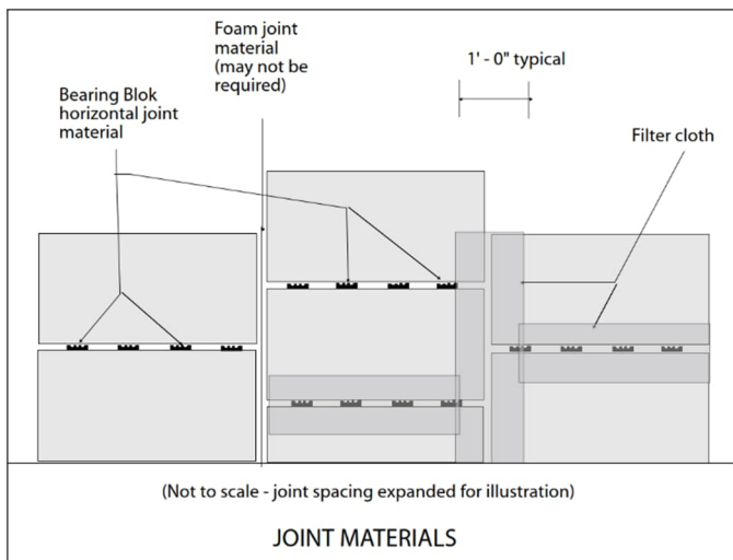
Figure 23: Joint material.
