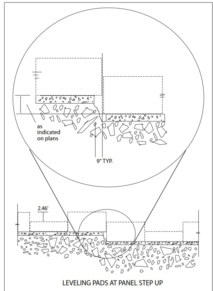
Figure 18: Leveling pad at panel step-up
