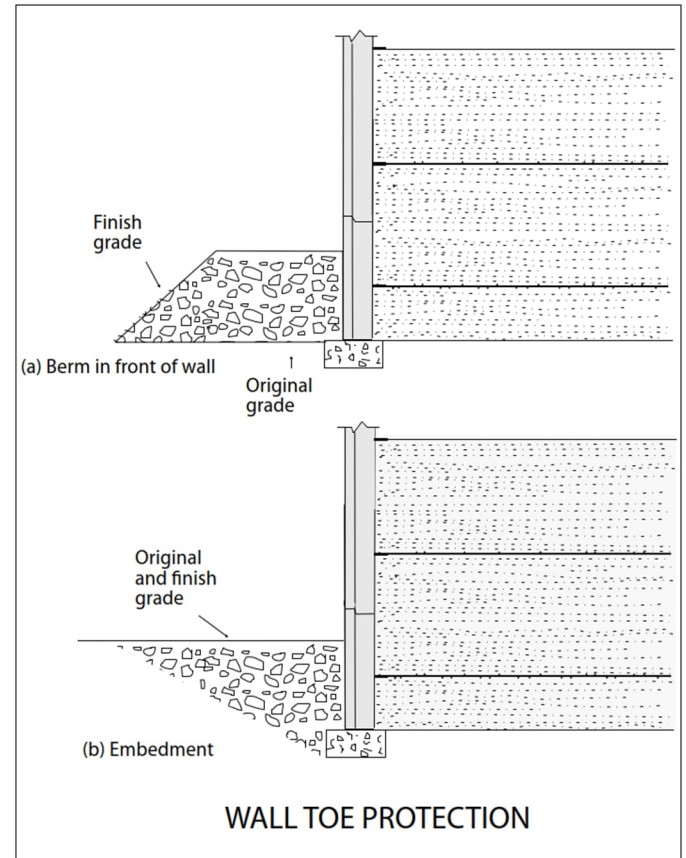
Figure 31: Wall toe protection.
