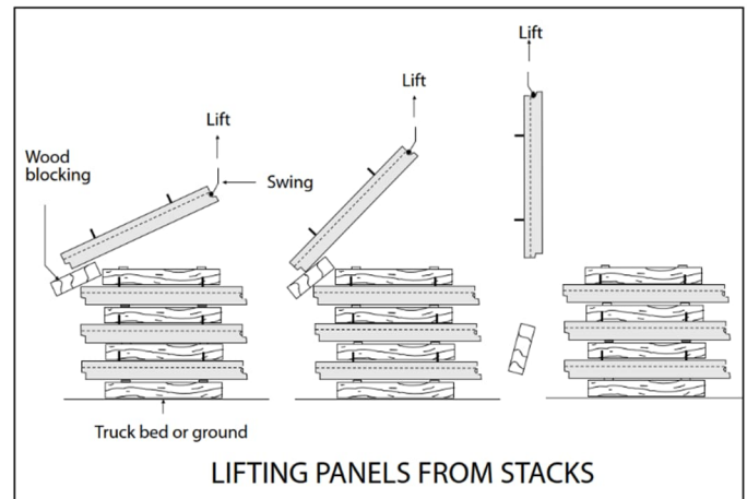
Figure 13: Lifting panels from a stack.
