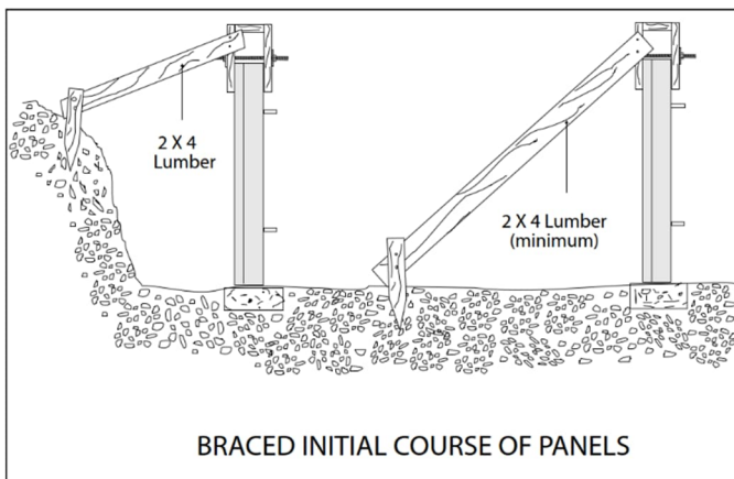
Figure 22: Panel bracing
