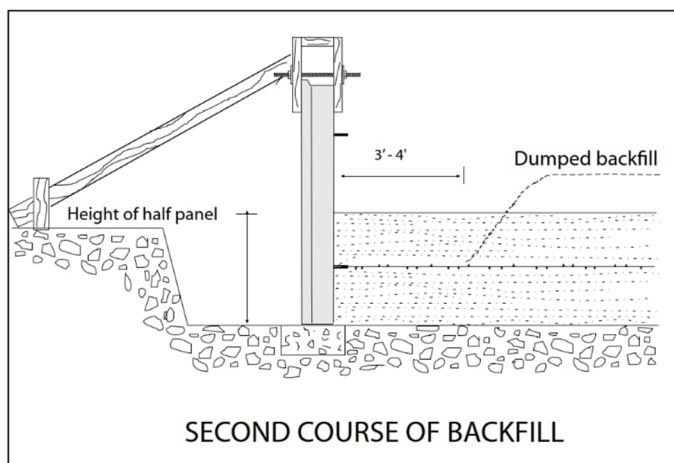
Figure 26: Second course of backfill.
