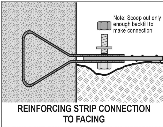
Figure 27: Reinforcing strip connection to facing.
