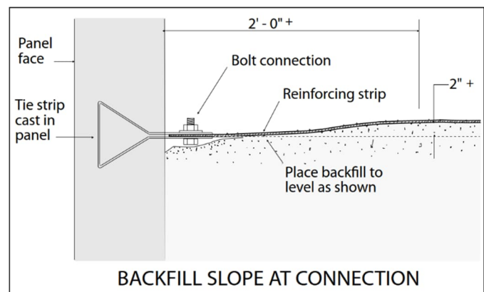
Figure 25: Backfill slope at connection.
