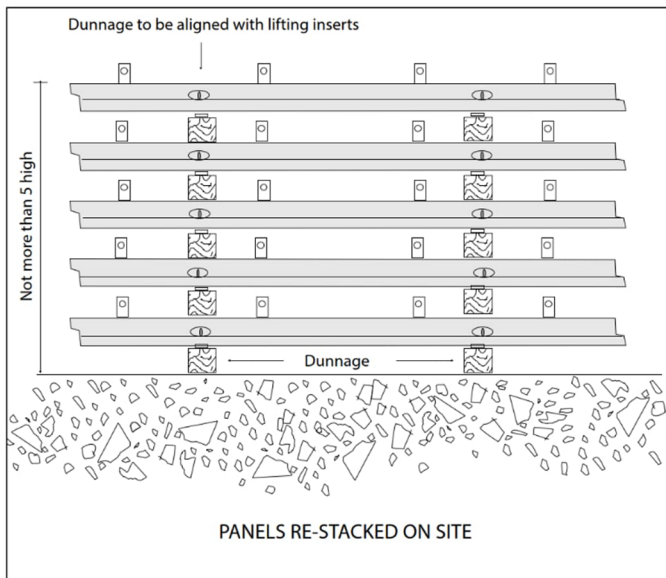
Figure 7: Panels re-stacked on site.
