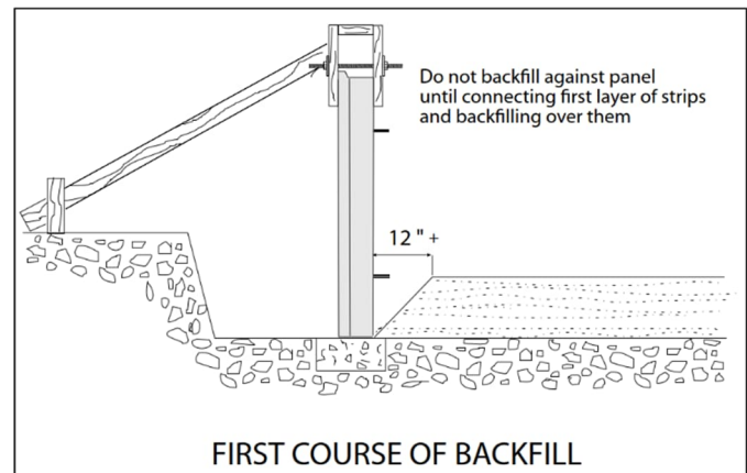
Figure 24: First course of backfill.
