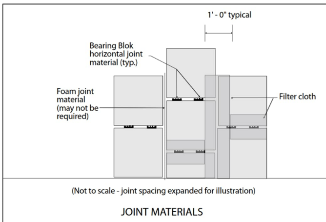
Figure 24: Joint material (Cruciform and Square panel types).
