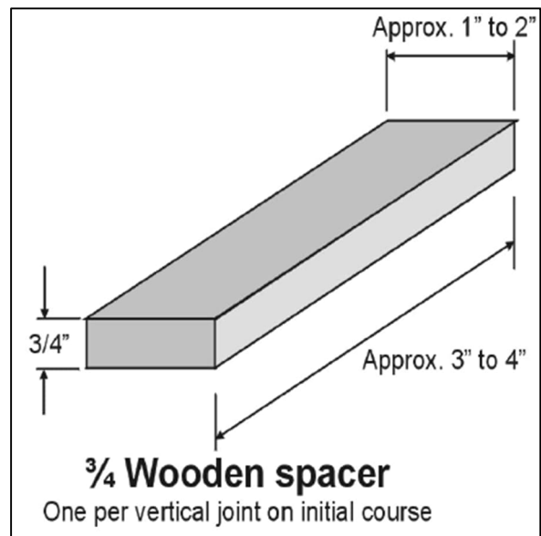
Figure 6: Wooden spacer.
