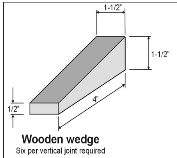
Figure 5: Wooden wedge.
