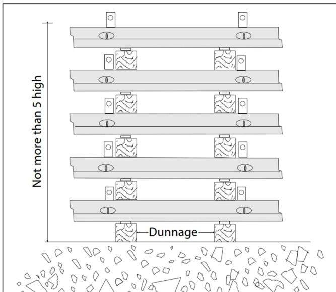
Figure 9: Panels re-stacked on site.
