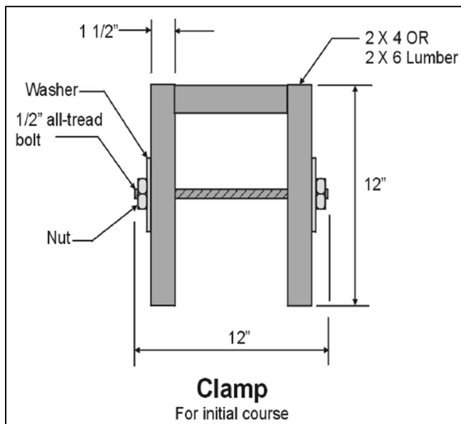
Figure 4: Clamp for initial panel course.
