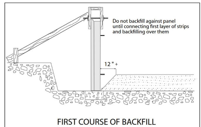
Figure 26: First course of backfill.
