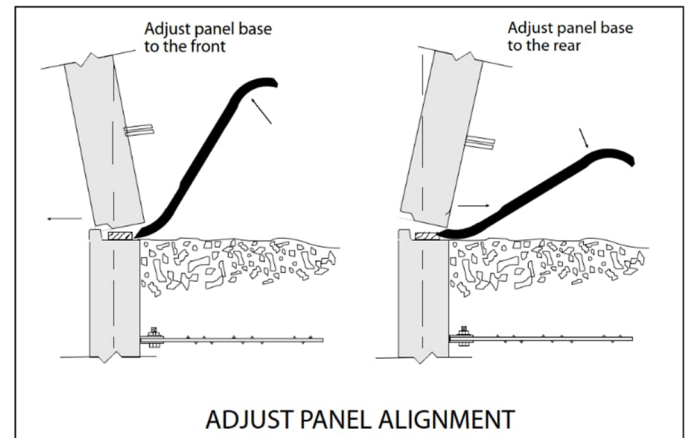
Figure 16: Adjusting panel alignment
