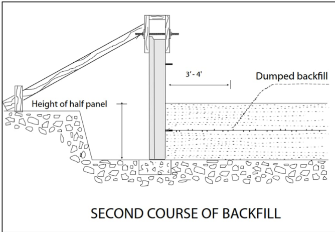
Figure 27: Second course of backfill.
