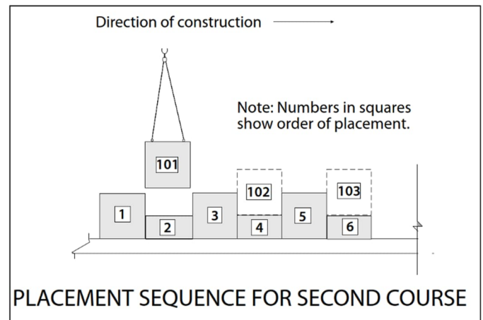
Figure 37: Placement sequence for second course.
