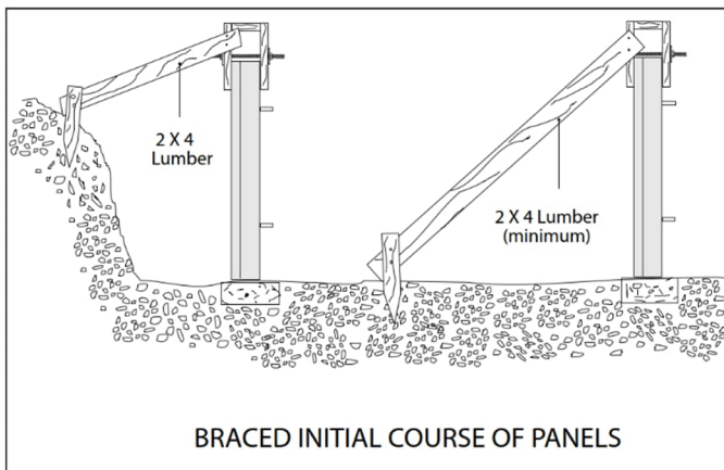
Figure 23: Panel bracing
