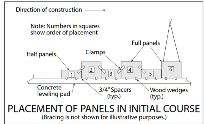
Figure 20: Placement of initial panel course (Square panel type shown here, similar for other panel types).
