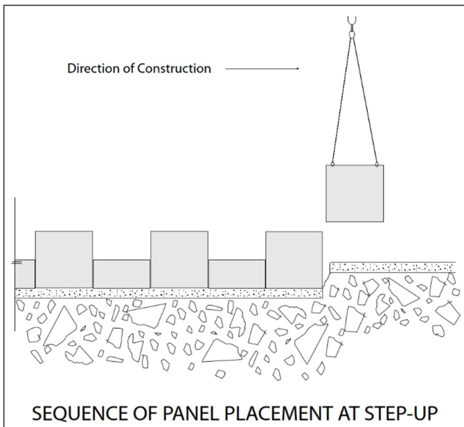
Figure 36: Sequence of panel placement at leveling pad step.
