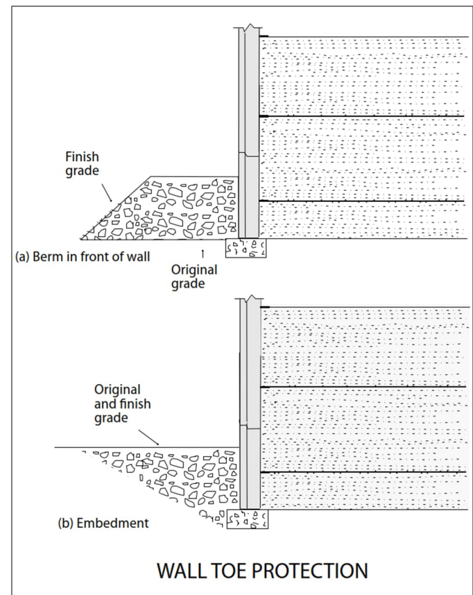
Figure 39: Wall toe protection.
