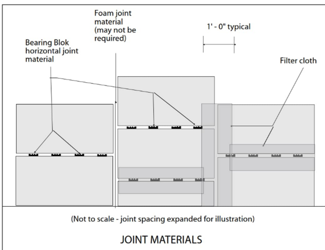
Figure 25: Joint material (Rectangular panel type).
