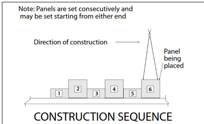
Figure 14: Use of spacer block to set panel spacing.
