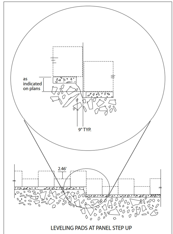
Figure 19: Leveling pad at panel step-up (Square panel type shown here, similar for other panel types).
