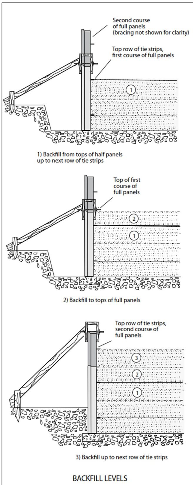
Figure 38: Backfill levels.
