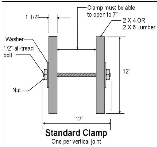
Figure 3: Standard clamp.
